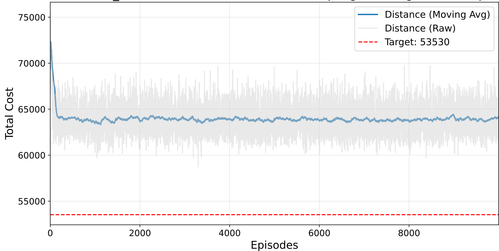
Final NO_MASK Masked AutoRL-SOP (Resampling) Training - ft70.4.sop
